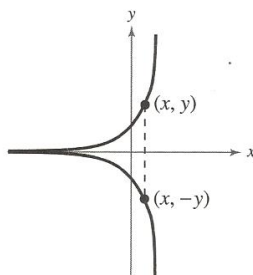
x-Axis Symmetry
